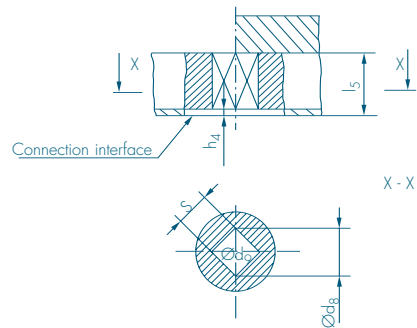
Actuator with diagonal square end
