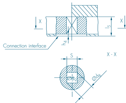
Actuator with parallel square end
