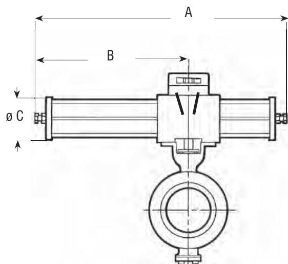
NAF 791294/791394
