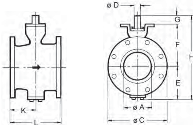
Flanged version
