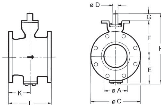
Flanged version
