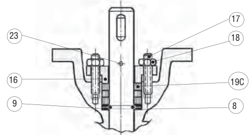
Stuffing box: Type -07, -17
