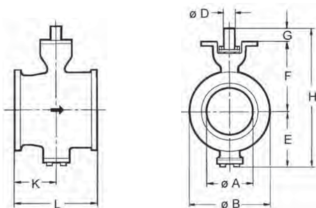
Wafer version
